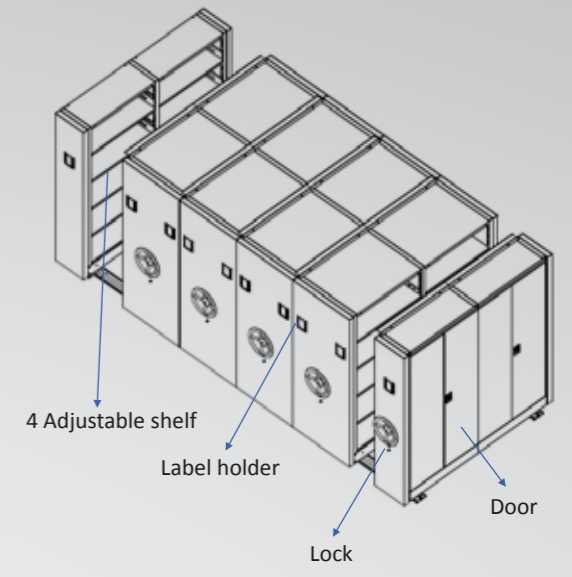
TWO BAY
