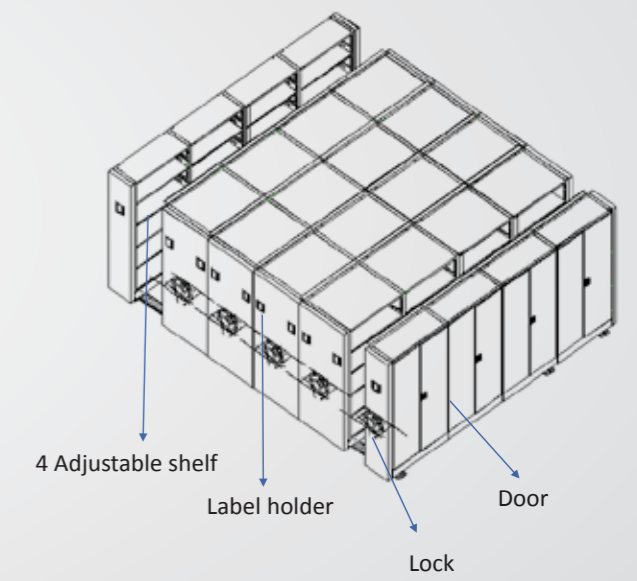
FOUR BAY
