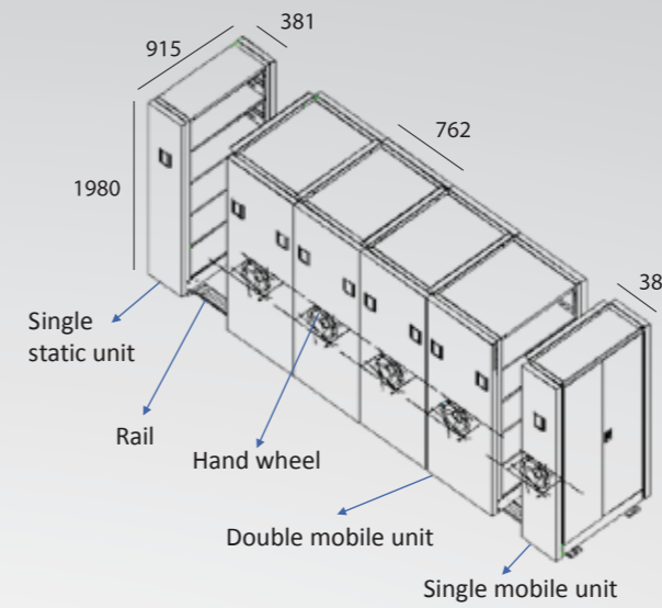
ONE BAY
